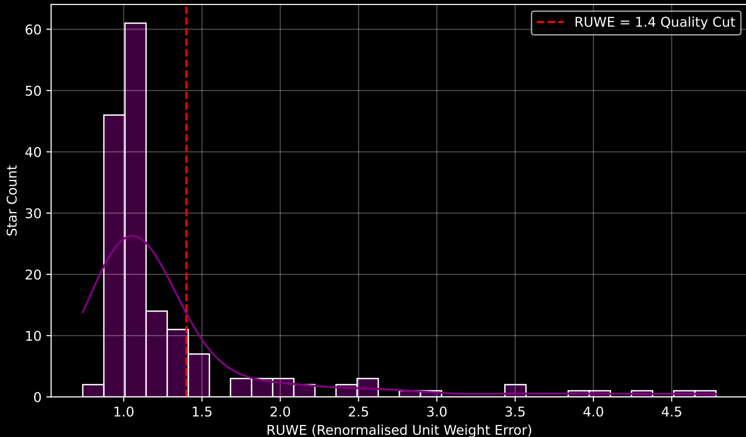
GAPOGEE DR17 Field [161+34_MGA] RUWE Distribution (n= 166)
