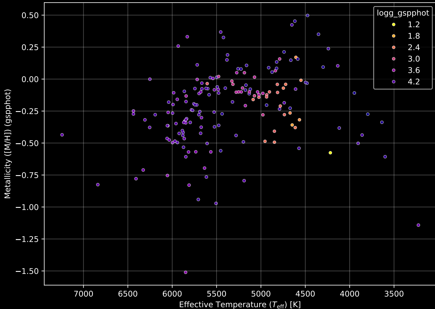
APOGEE DR17 Field: [161+34_MGA] Stellar Population Parameters (n= 173)
