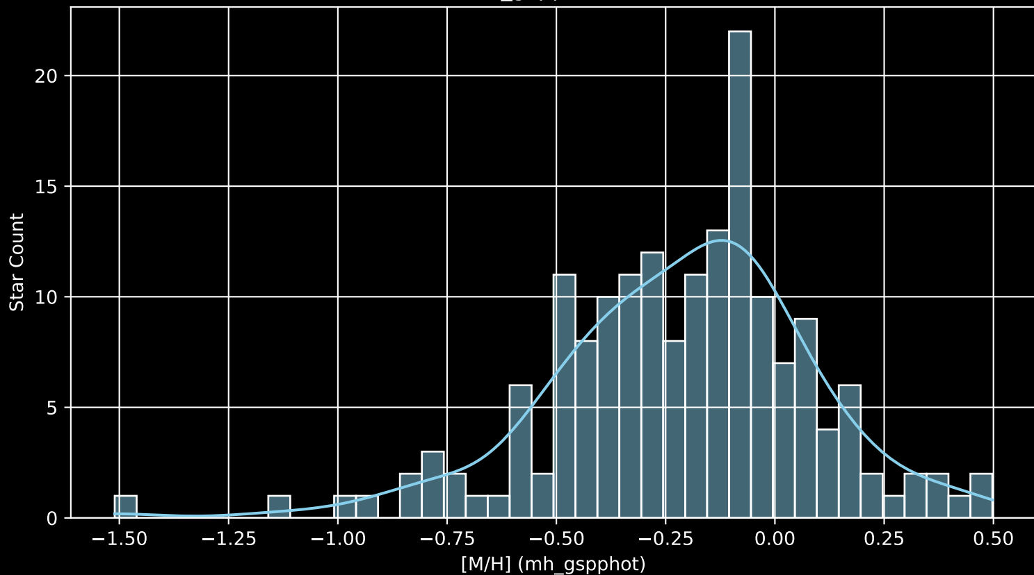
APOGEE DR17 Field: [161+34_MGA [M/H] (mh_gspphot) (n= 173)
