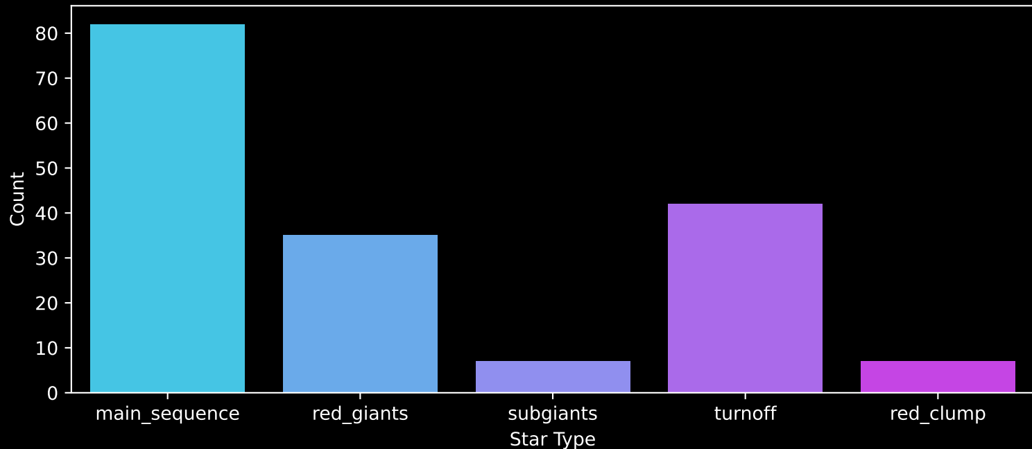
APOGEE DR17 Field: [161+34_MGA] Count plot of Star Type
