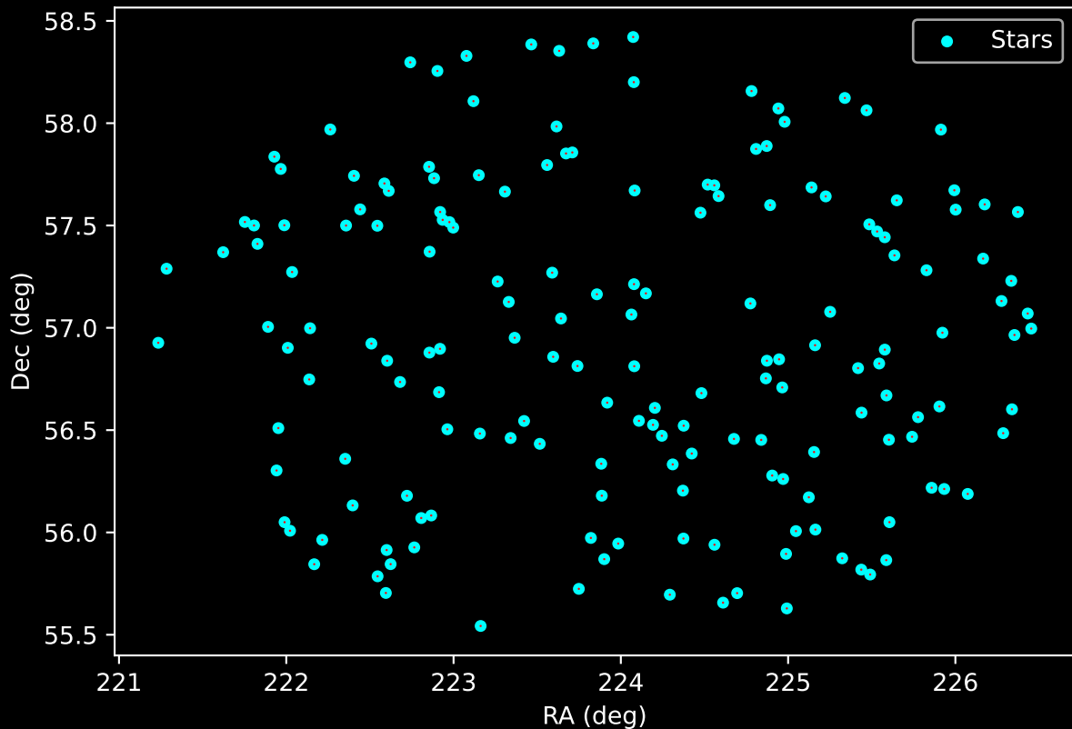
APOGEE DR17 Field: [161+34_MGA] Proper Motion Vectors for Gaia Star Field (n= 173)
