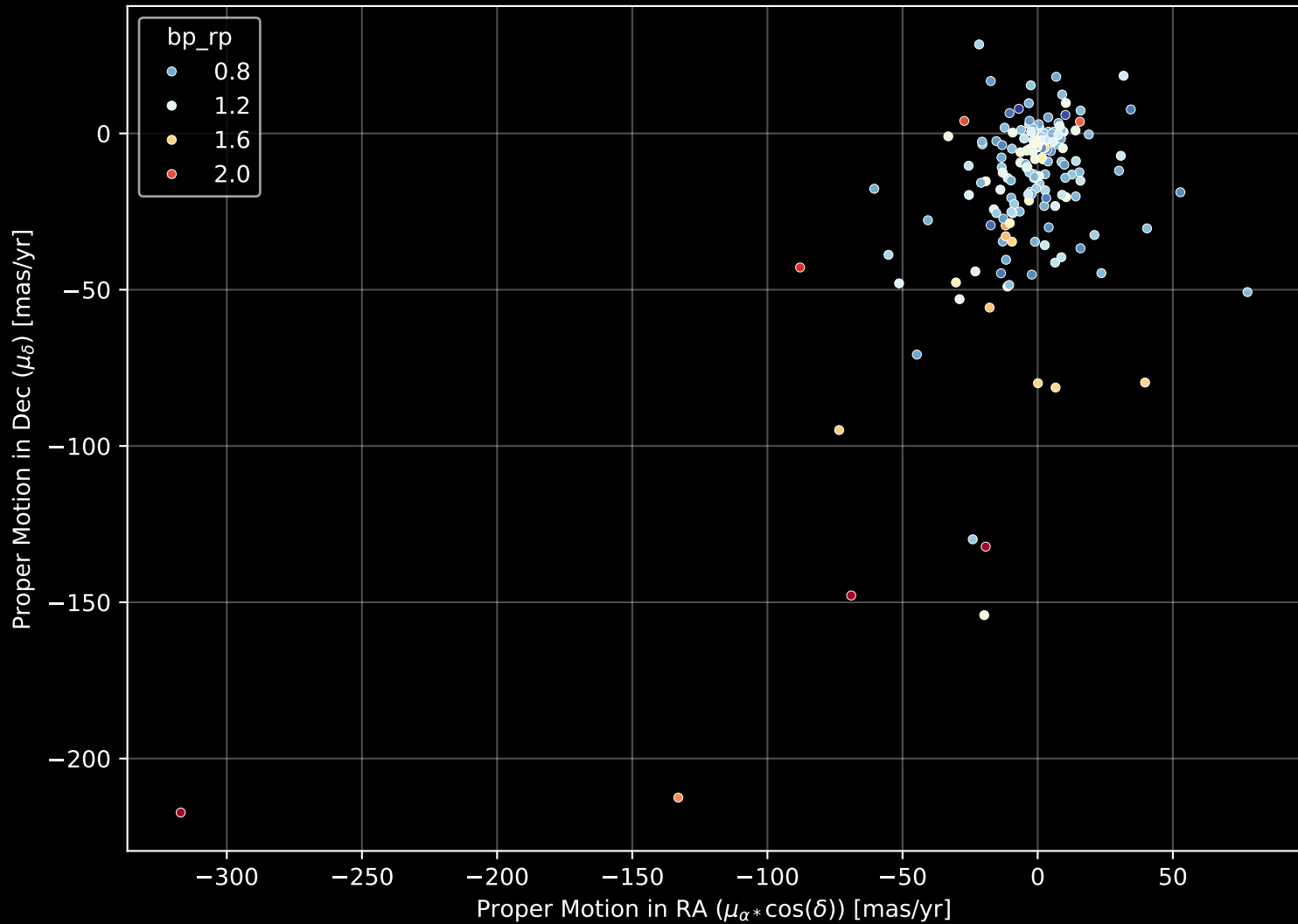
APOGEE DR17 Field: [161+34_MGA] Proper Motion Diagram (n= 173)
