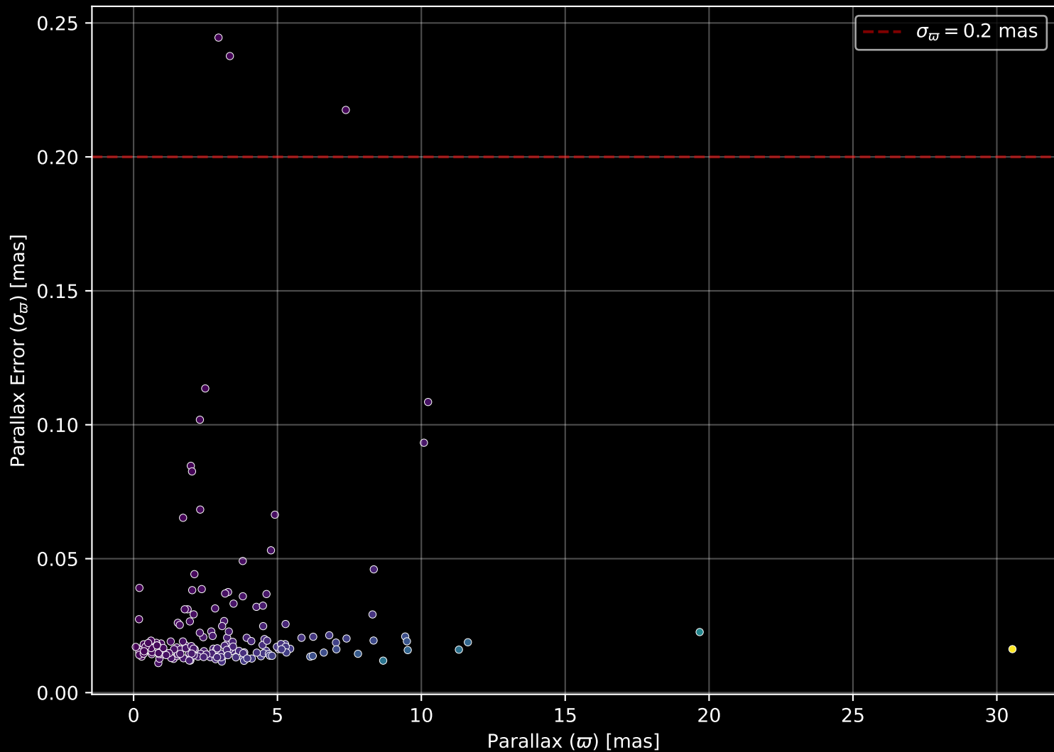
APOGEE DR17 Field: [161+34_MGA] Parallax Quality (n= 173)
